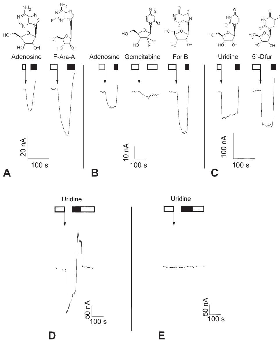
Fig. 1. Interaction of nucleoside-derived drugs with the rat Na + -dependent concentrative nucleoside transporter CNT2 (rCNT2). A–C: rCNT2-expressing oocytes were held at -50 mV of membrane potential and perfused with Na + buffer in the absence of substrate (open box), and current was continuously recorded (baseline current). A: addition of 1 mM adenosine (arrow) induced an inward current of 20 nA. The oocyte was then washed out with Na + -free buffer (filled box), which blocked the adenosine inward current and the baseline current. After the perfusion with Na + buffer, the current returned to baseline. The addition of 1 mM fludarabine (F-Ara-A) induced an inward current 2-fold higher than adenosine current, indicating that it is transported. B: in a different oocyte the current induced by 1 mM formycin B (For B) was also double the current induced by 1 mM adenosine. Gemcitabine (1 mM) induced a very small current. C: 1 mM 5-fluoro-5'-deoxyuridine (5'-Dfur) induced higher inward current than 0.5 mM uridine. D: a rCNT2-expressing oocyte was held at -50 mV of membrane potential and perfused with Na + buffer in the absence of substrate (open box), and current was continuously recorded (baseline current). The addition of 0.5 mM uridine induced an inward current of \sim 200 nA. This current and the baseline current disappeared when the oocyte was washed out with Na + -free buffer (filled box). The oocyte was then perfused with Na + buffer, and the baseline current was restored; this current is referred to as the Na + -leak current. E: in a noninjected oocyte from the same batch as the oocyte in D, no uridine-induced current or Na + -leak current was obtained.
