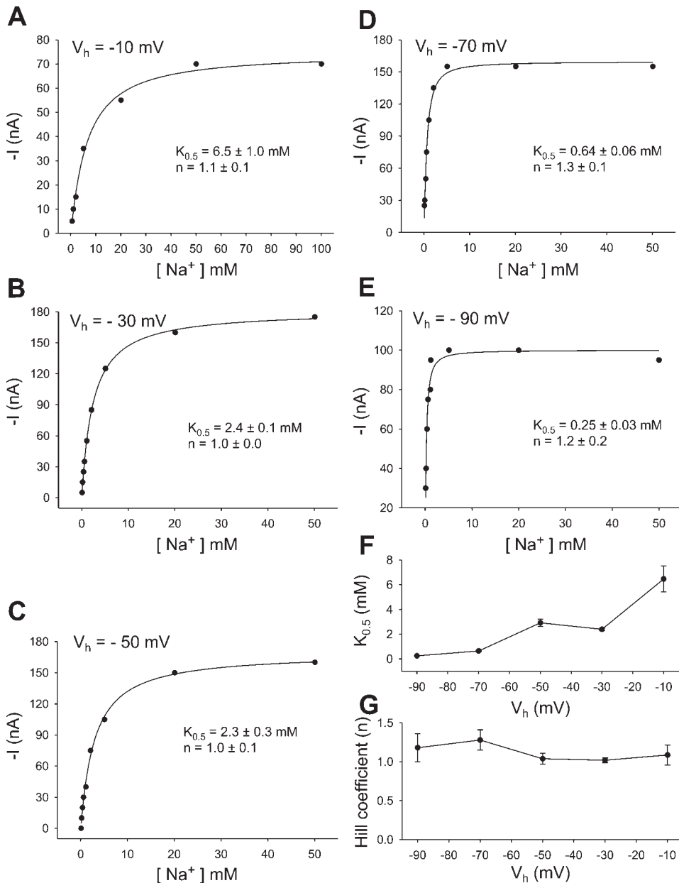
Fig. 5. \text{Na}^+ activation curves at different membrane potential ( V_h ). A–E: K_{0.5}^{\text{Na}^+} was obtained by fitting the currents at each \text{Na}^+ concentration to Eq. 1 in MATERIALS AND METHODS. Each curve corresponds to a single representative rCNT2-expressing oocyte. Similar results were obtained with oocytes from 3 different batches. F: K_{0.5}^{\text{Na}^+} as a function of V_h . G: Hill coefficient as a function of V_h .
