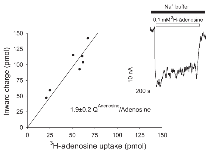
Fig. 6. Charge-to-nucleoside stoichiometry for rCNT2. Inset : a representative experiment showing 0.1 mM [ ^3\text{H} ]adenosine-induced inward current in a rCNT2-expressing oocyte. Membrane potential was held at -50 mV, and the oocyte perfused with \text{Na}^+ buffer until a stable baseline current was recorded. The addition of 0.1 mM [ ^3\text{H} ]adenosine increased the inward current to \sim 18 nA during 9 min of perfusion. Adenosine was then removed from the bath by perfusing adenosine-free \text{Na}^+ buffer, and the current returned to baseline. The transported charge, Q , was calculated as the integral of the adenosine-dependent current over the 9-min period and was 9.9 \times 10^{-6} C. The [ ^3\text{H} ]adenosine uptake in this oocyte was 62 pmol after subtraction of [ ^3\text{H} ]adenosine uptake, over the same period, in a noninjected oocyte. Uptake of 0.1 mM [ ^3\text{H} ]adenosine in the presence of 100 mM \text{Na}^+ and the induced current were measured for 5–10 min in 7 different oocytes as indicated in the inset . The adenosine-dependent charge ( Q^{\text{adenosine}} ) for each oocyte was plotted against the uptake of adenosine in the same oocyte. The data were fitted to a linear regression with a slope of 1.9 \pm 0.2 charges/adenosine.
