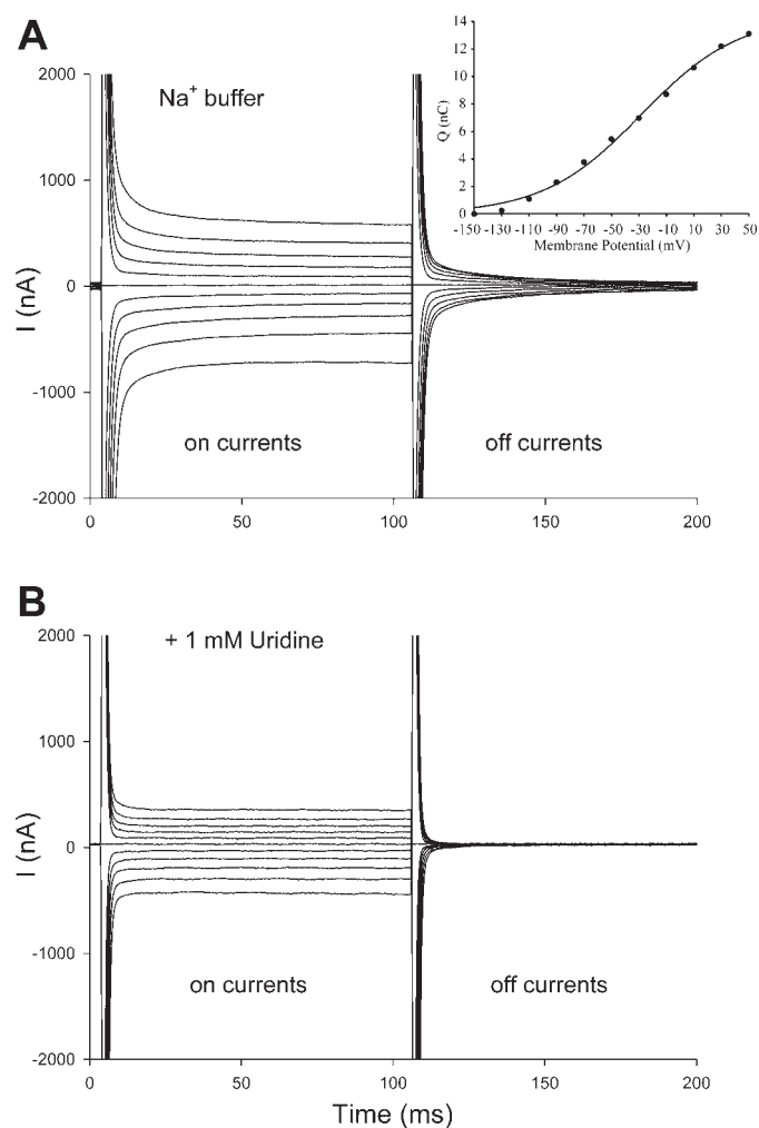
Fig. 7. Membrane current records of rCNT2. A : a rCNT2-expressing oocyte was held at -50 mV and stepped to 11 test values between +50 and -150 mV ( -20 mV decrement). In \text{Na}^+ buffer and in the absence of uridine, the oocyte showed pre-steady-state currents in response to step changes in the membrane voltage and showed steady-state currents due to the \text{Na}^+ leak through the transporter. B : the addition of 1 mM uridine blocked the pre-steady-state currents and caused an increase of the steady-state inward currents. Inset : charge-voltage relationship for a representative oocyte expressing rCNT2. The data ( \bullet ) were obtained as described in MATERIALS AND METHODS and fitted to the Boltzmann equation (solid line, Eq. 2) from which a V_{0.5} of -28 \pm 5 was calculated.
