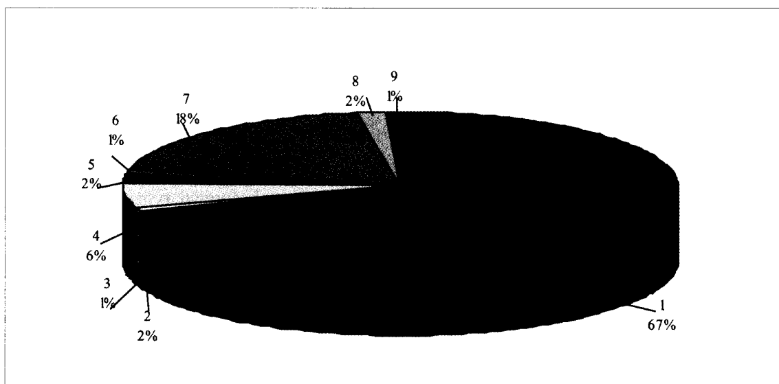
Fig. 1. Percentage of abundance of ectomycorrhizal morphotypes; 1: Cenococcum geophilum ; 2: T. brumale ; 3: T. albidum ; 4: Hebeloma ; 5: Hymenogaster ; 6: SB type; 7: Type 1; 8: Type 2; 9: Type 3.
