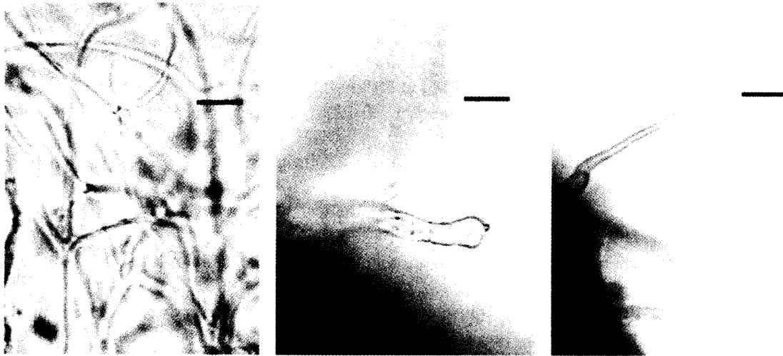
Fig. 2. Unidentified morphotypes of ectomycorrhizae (bars= 0,01 mm); a: Type 1; b: Type 2; c: Type 3.
