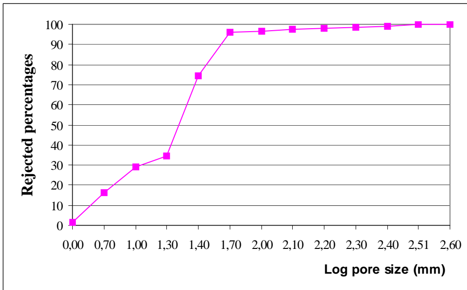
Figure 4. Granulometric curve MC1.
