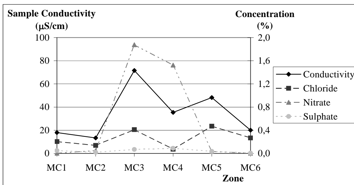
Figure 3. Results of sample conductivity and anions concentration determined by ion chromatography (Conductivity, expressed in \mu\text{S}\cdot\text{cm}^{-1} is given for a suspension of 1 mg of the sample per mL. The concentrations of anions are expressed as percentages of the samples).
