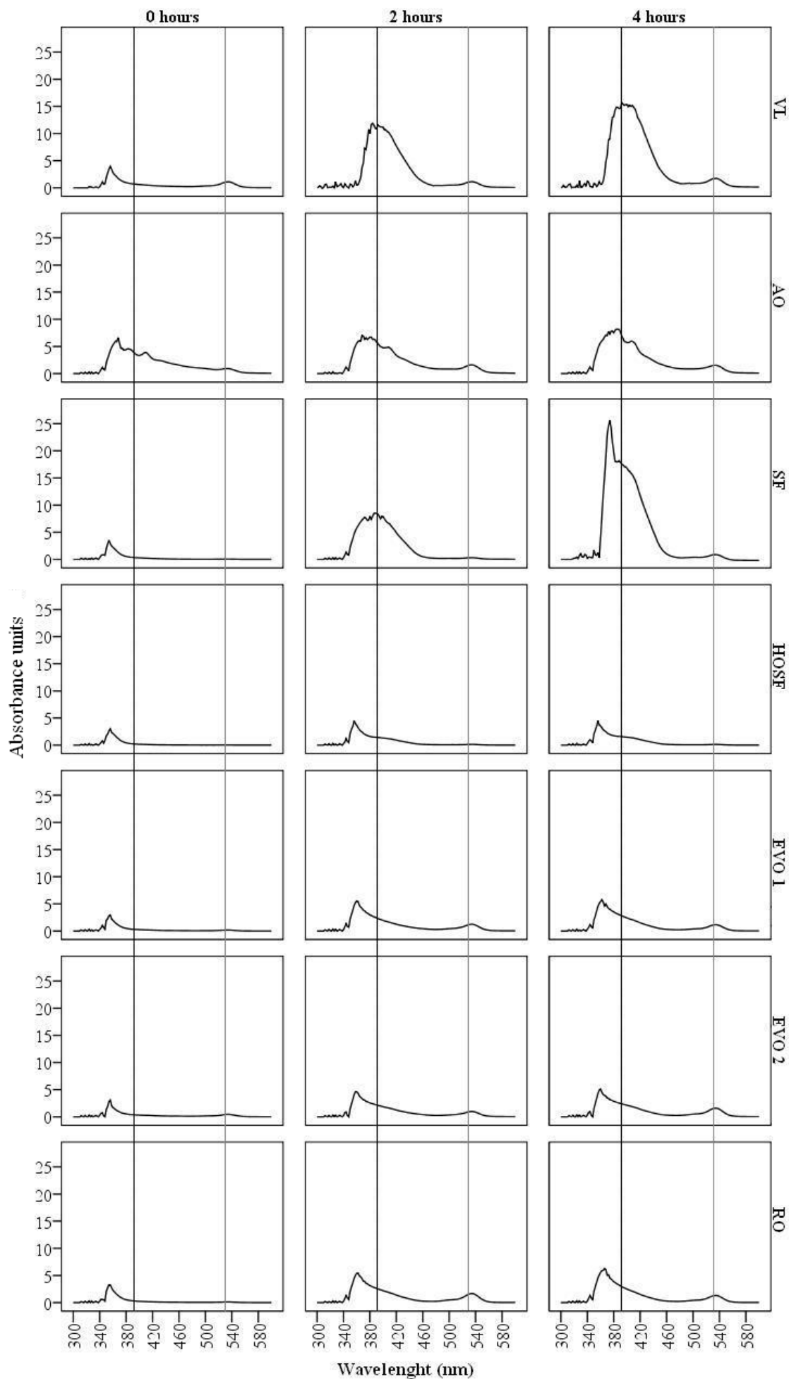
Figure 1. Absorption spectra of the seven oils studied. During the heating process (180°C, 0, 2 and 4 hours) (VL, virgin linseed oil; AO, algae oil; SF, sunflower oil; HOSF, high-oleic sunflower oil; EVO, extra virgin olive oil; RO, refined olive oil).
