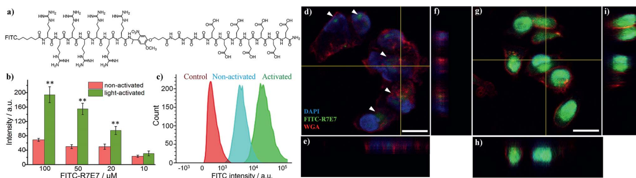
Fig. 2 (a) Structure of the FITC-labelled photo-cleavable peptide (FITC-R7E7). (b) Cellular uptake of FITC-R7E7 by MDA-MB-231 cells at different concentrations ( i.e. , 100, 50, 20 and 10 \mu\text{M} ) before and after light activation for 10 min was evaluated by quantifying cellular fluorescence intensity. (c) FACS data and (d–i) confocal images of MDA-MB-231 cells highlight the distinct difference in FITC internalization when cells were incubated with 50 \mu\text{M} FITC-R7E7 in the absence of (d–f) and following (g–i) light irradiation. Scale bar: 20 \mu\text{m} . **: p < 0.01 non-activated vs. activated. The nucleus is stained with DAPI (4',6-diamidino-2-phenylindole, dihydrochloride); the plasma membrane is stained with the probe WGA (wheat germ agglutinin).
